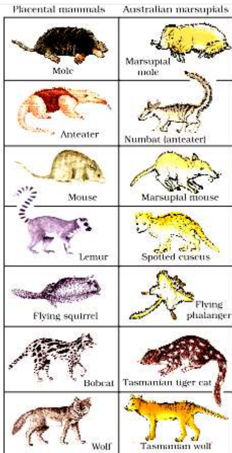
Fig: Picture showing convergent evolution of Australian Marsupials and placental mammals
